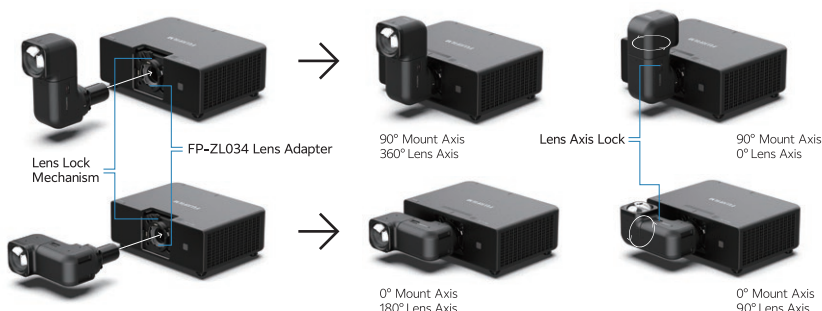
FP-ZL034 Ultra Short Throw 1.2x Zoom Lens Installation Image
