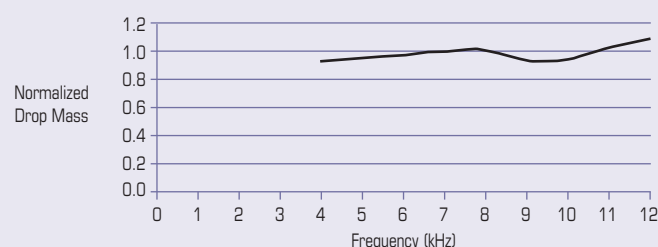
Galaxy PH 256/80 HM Typical Drop Mass vs. Frequency
