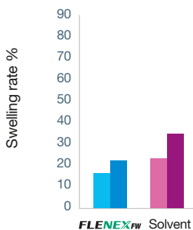
In 12 and 24 hour plate swell tests, Flenex FW resulted in 25% to 45% less swelling compared to solvent plates.
